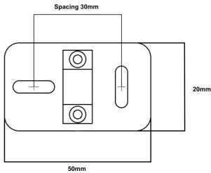
Dimensions of mounting support
